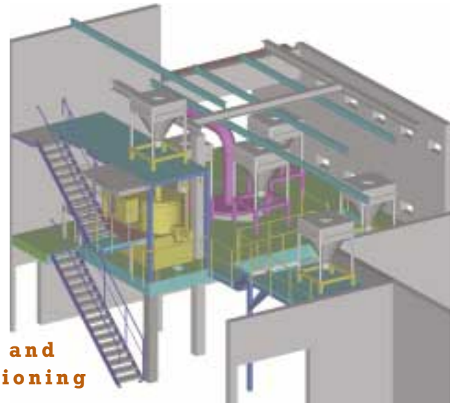
Detail engineering/commissioning - feeding system production plant
